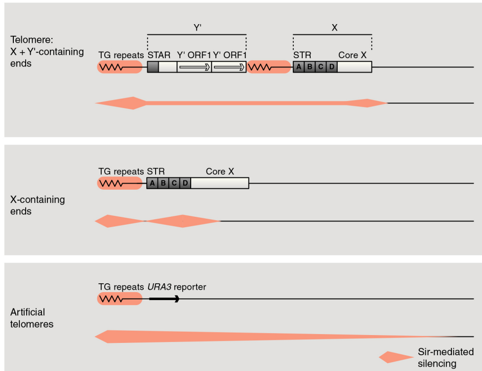
Figure 10. The organization of native telomeres and their silencing patterns. Subtelomeric elements are shown with their major protein binding sites. Telomeres fall into the two general classes: X-containing or X+Y'-containing ends. The STAR and STR elements block the propagation of repression and leave a region of reduced repression within the Y' or X element. This is not the case at artificially truncated telomeres in which there is a gradient of repression that extends 3–4 kb from the TG repeat. Looping similar to that in Figures 5 and 6 is proposed for native telomeres, so that repressed regions contact each other leaving unrepressed chromatin in between areas of contact. (Adapted from Pryde and Louis 1999.)
